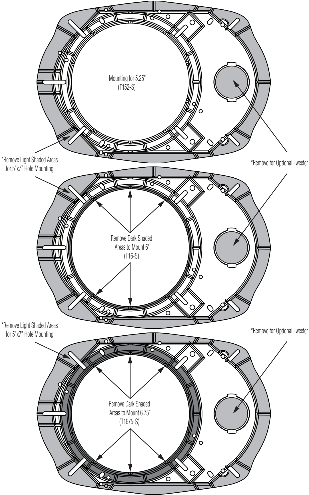
Adapter Plate Template - 6"x9" Hole Mounting
