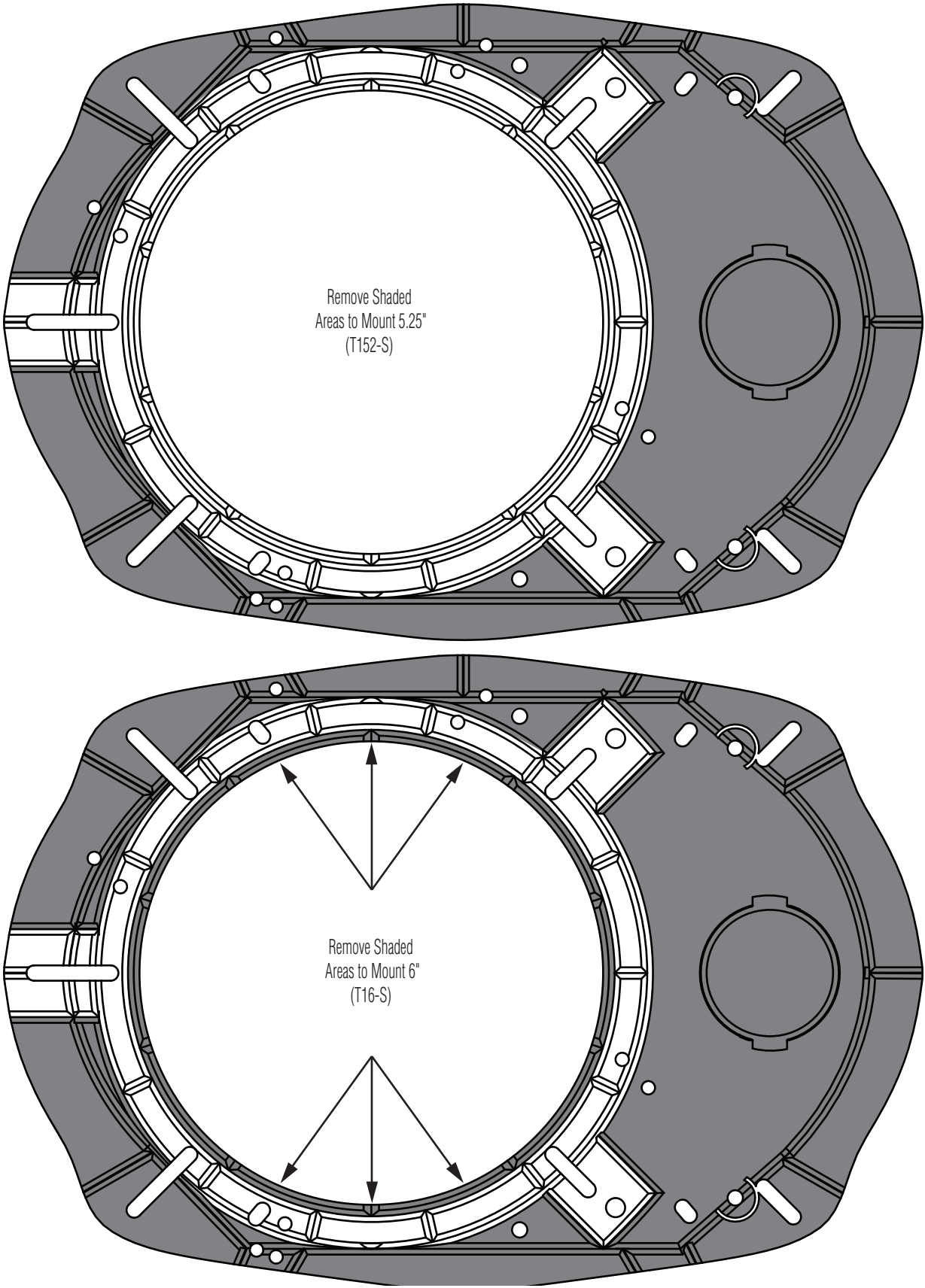
Adapter Plate Template - 6.75" Hole Mounting
